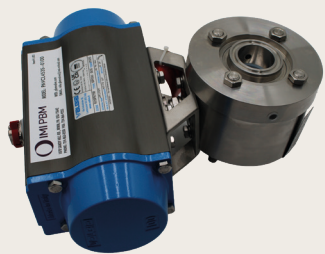
Angle Stem Flush Tank Ball Valves Sizes 1" to 6" (DN25 - DN150)
