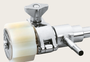
Rising Stem Sampling Valves Size ¼" Bore Diameter
