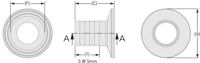
Type A – 25.0mm Flange
