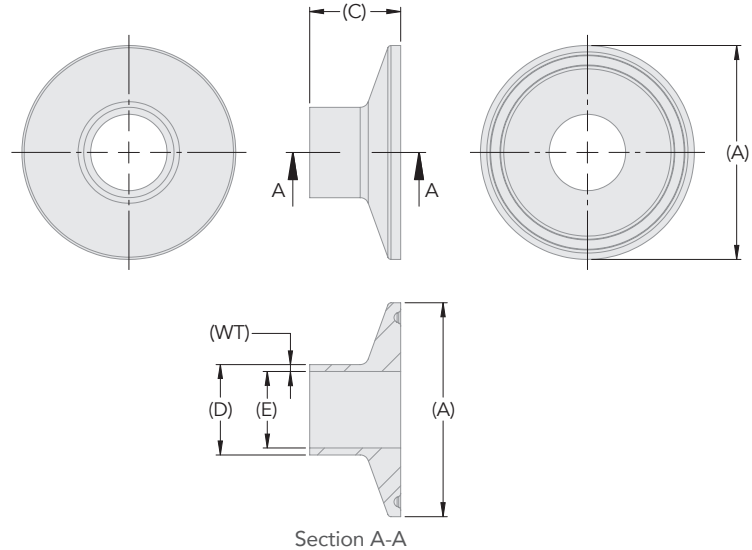
Type B – 50.5mm to 338.0mm Flange
