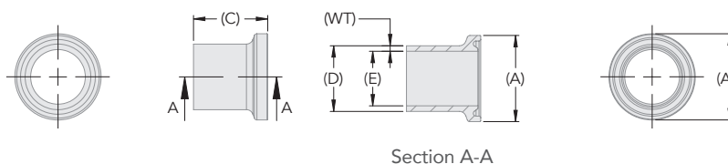
Type B – 50.5mm to 338.0mm Flange
