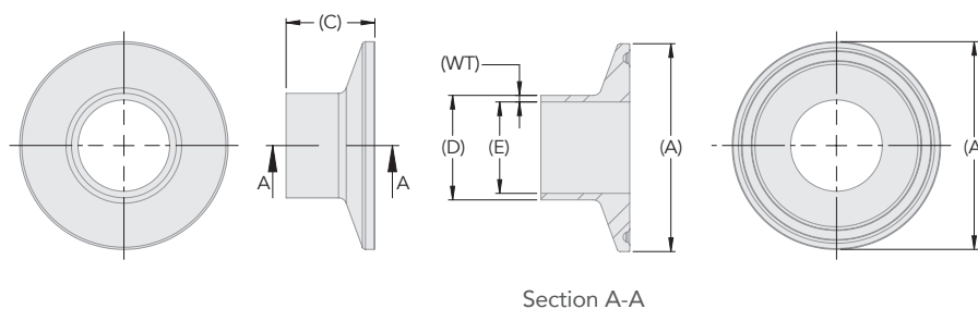
Type B – 50.5mm to 119.0mm Flange
