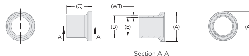
Type B – 34.0mm to 233.5mm Flange
