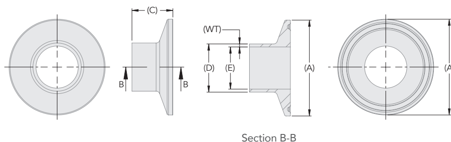
Type B – 50.5mm to 338.0mm Flange
