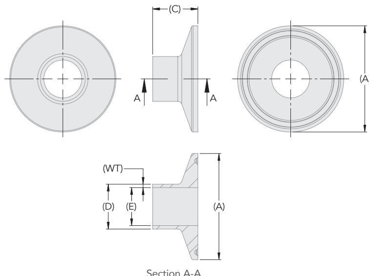
Type B – 50.5mm to 338.0mm Flange
