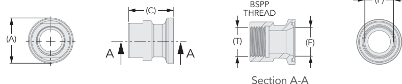
Type B – 50.5mm to 64.0mm Flange
