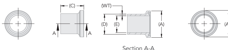
Type B – 34.0mm to 233.5mm Flange
