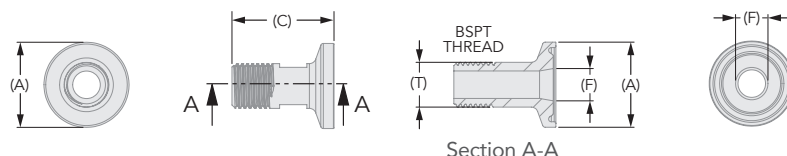
Type B – 50.5mm to 64.0mm Flange
