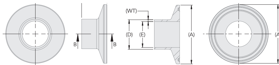
Section B-B
