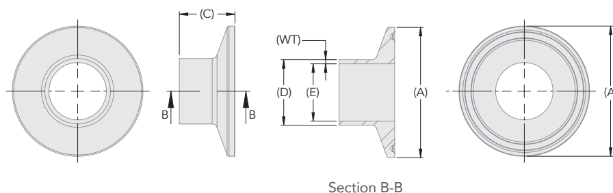
Type B – 50.5mm to 167.0mm Flange
